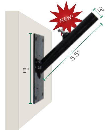
Flag Pole Holder Only [No. 345]
